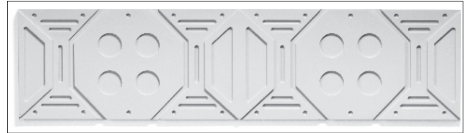
PD 141 Space Panel 1990mm x 500mm x 35mm
