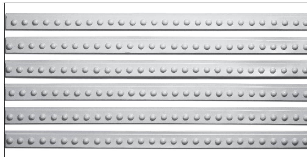
PD 63 Rivet Strips Sheet size: 2320mm x 1250mm x 40mm Rivets 45mm dia, Strips 130mm wide
