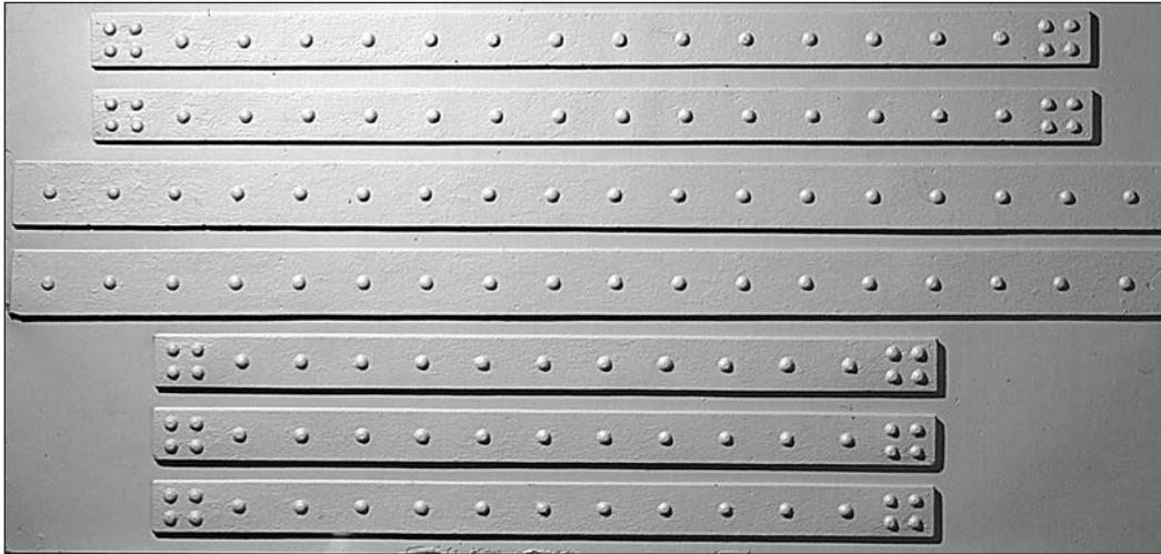
7 Metal riveted straps width 100mm Panel size: 2320mm x 1050mm x 25mm
