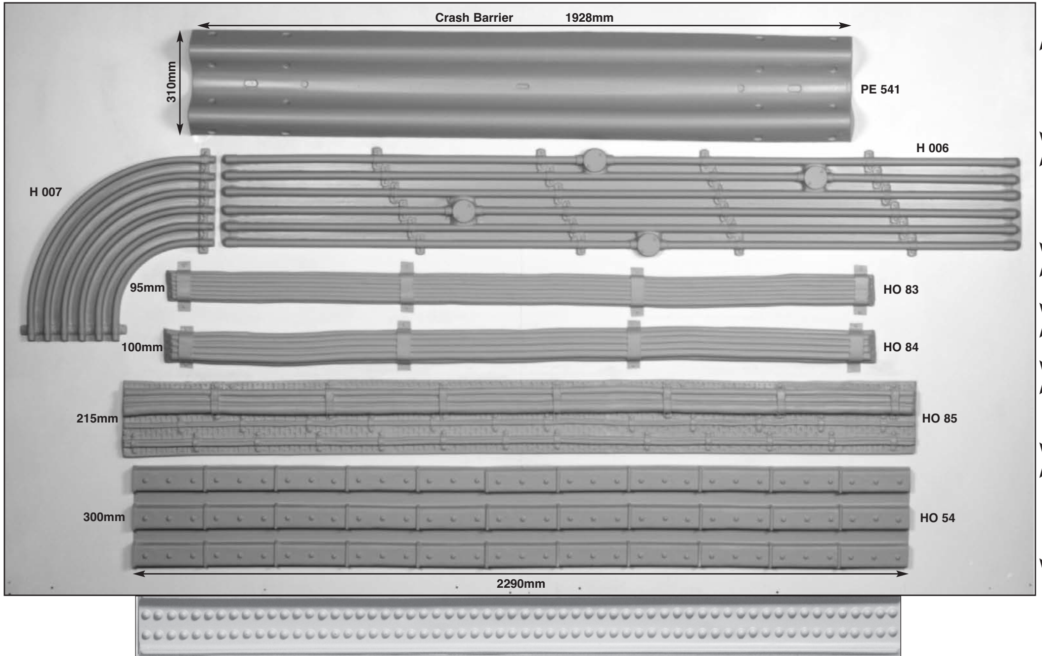
PE 005 Riveted Beam 2295mm x 190mm x 55mm Individual Rivets 25mm Dia
