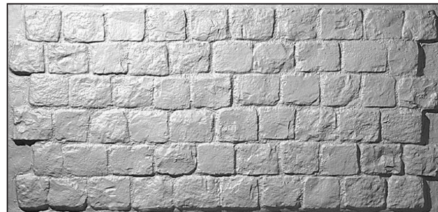
S 92 French cobblestones Cobble size: 150mm x 160mm Panel size: 2110mm x 1015mm x 14mm
