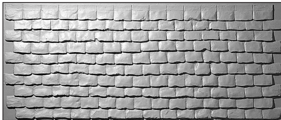
PD 15 Rustic English tiles - Tile size: 130mm x 85mm Panel size: 2240mm x 900mm x 25mm
