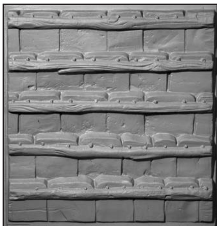
E 005 Peg tiles underside Panel size: 1143mm x 1092mm x 64mm
