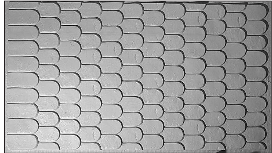
PE 516 Half round tiles Tile size: 110mm x 165mm Panel size: 1900mm x 1080mm x 16mm
